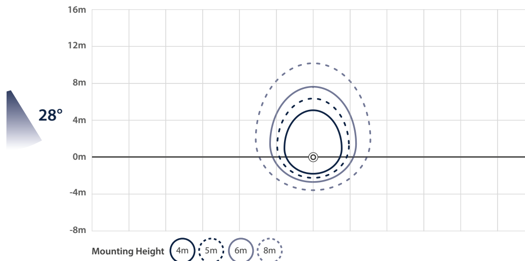
SmartScan External Sensor - Detection Area - 28°
